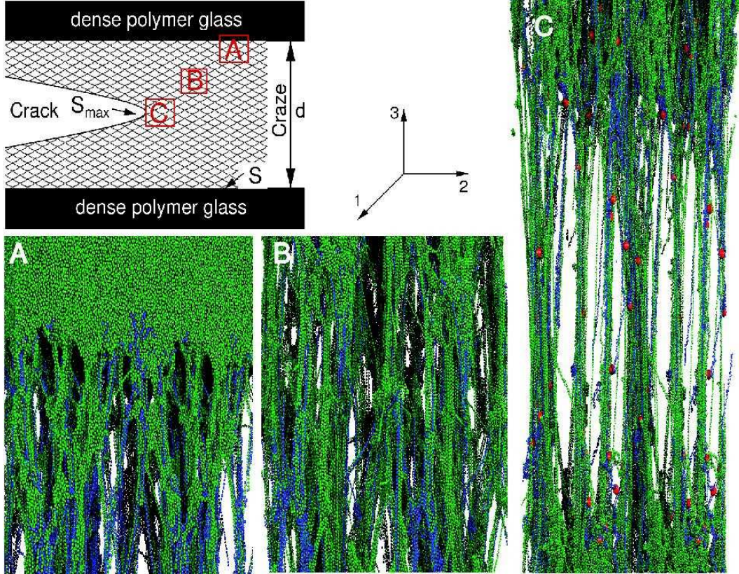
FIG. 1. Some length scales involved in the fracture of glassy polymers. A \sim mm long crack penetrates the material. A craze of typical width d = 10 - 50\mu\text{m} and length l \sim 10d forms in the “process zone” in front of the crack tip (top left). Craze formation (A), deformation (B) and failure (C) are studied with molecular dynamics simulations of \sim 100 nm-sized volume elements. A: craze fibrils emerge from the dense polymer glass (top) within a narrow “active zone”, B: fully developed craze structure, C: failure of the craze immediately in front of the crack tip. Individual beads of the polymer chains are shown as small ellipsoids. Chains carrying the largest tension are colored blue and broken bonds in C are colored red. The width of each image is 128 bead diameters. The fibril spacing D_0 is \sim 10 bead diameters for this figure, but depends on temperature, chain rigidity and other parameters.
